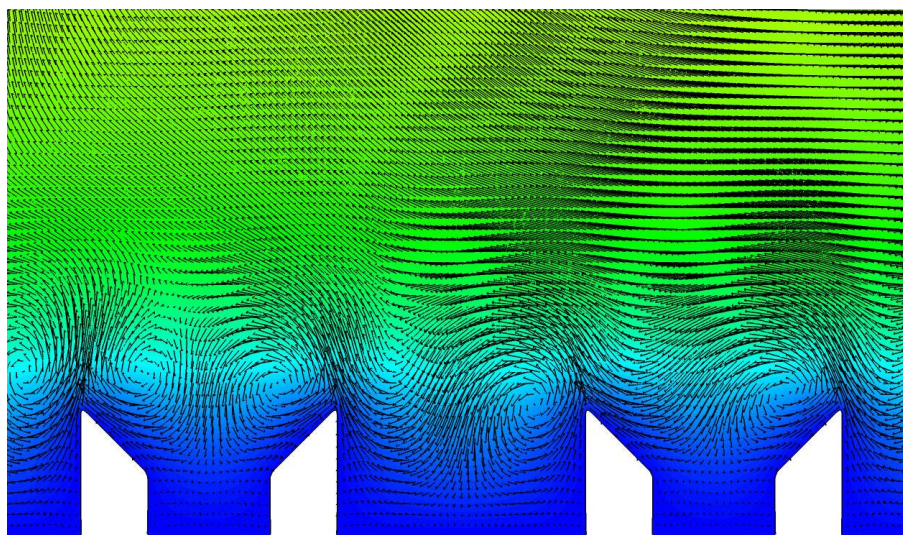
Fig. 1: Contours of the streamwise velocity together with the velocity vectors in the blade-type riblet DNS at Re_{\tau}=395 .
