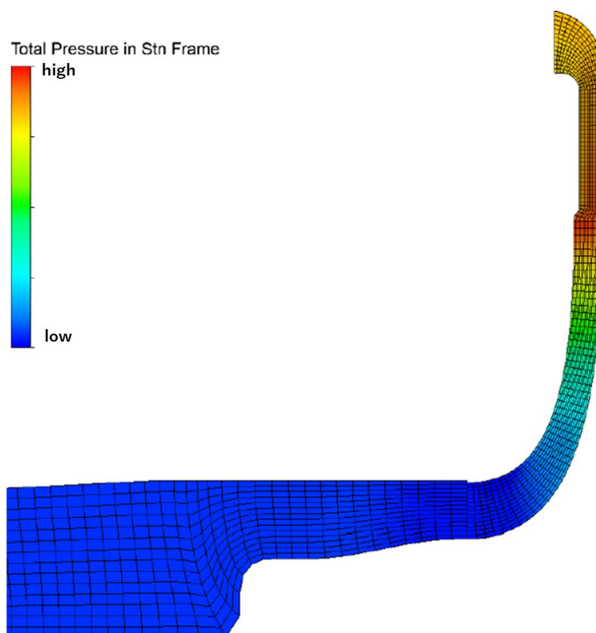
Fig. 1: Liquid hydrogen pump meridian pressure contour diagram
