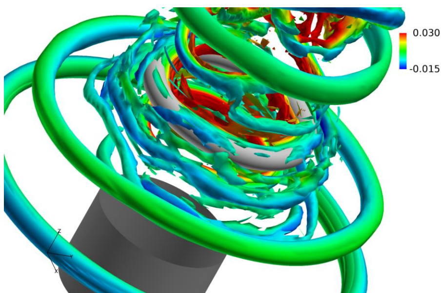
Fig. 1: Interaction between vortices extracted by the iso-surfaces of Liutex and the ring
