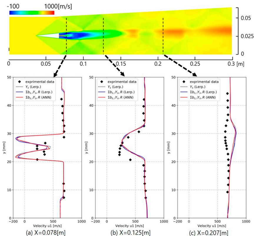
Fig. 1: Axial velocity distribution (experiment, conventional method A, method B, ANN method C)
