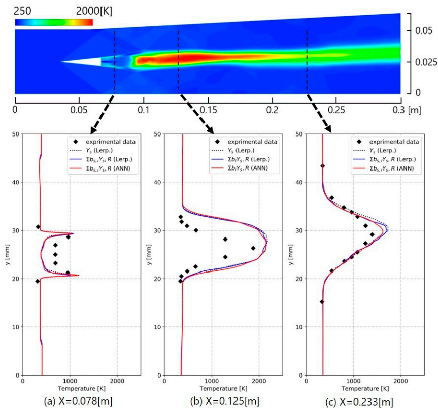
Fig. 2: Temperature distribution (experiment, conventional method A, method B, ANN method C)
