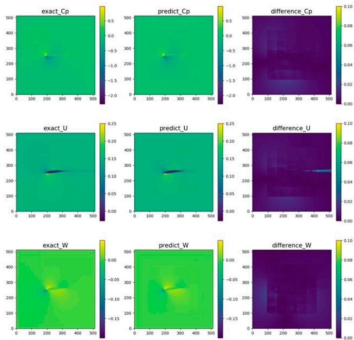
Fig. 2: Prediction result for trained data
